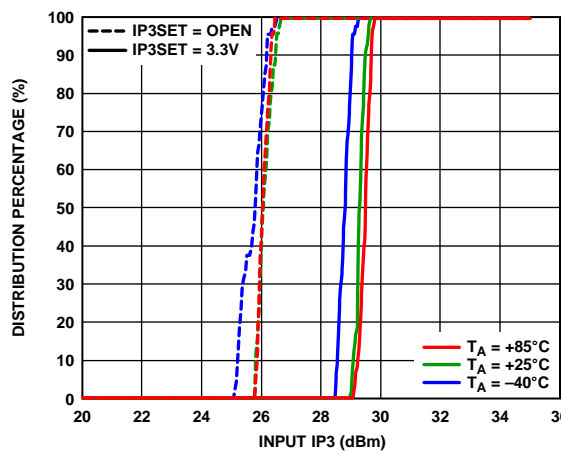
Figure 29. Input IP3
